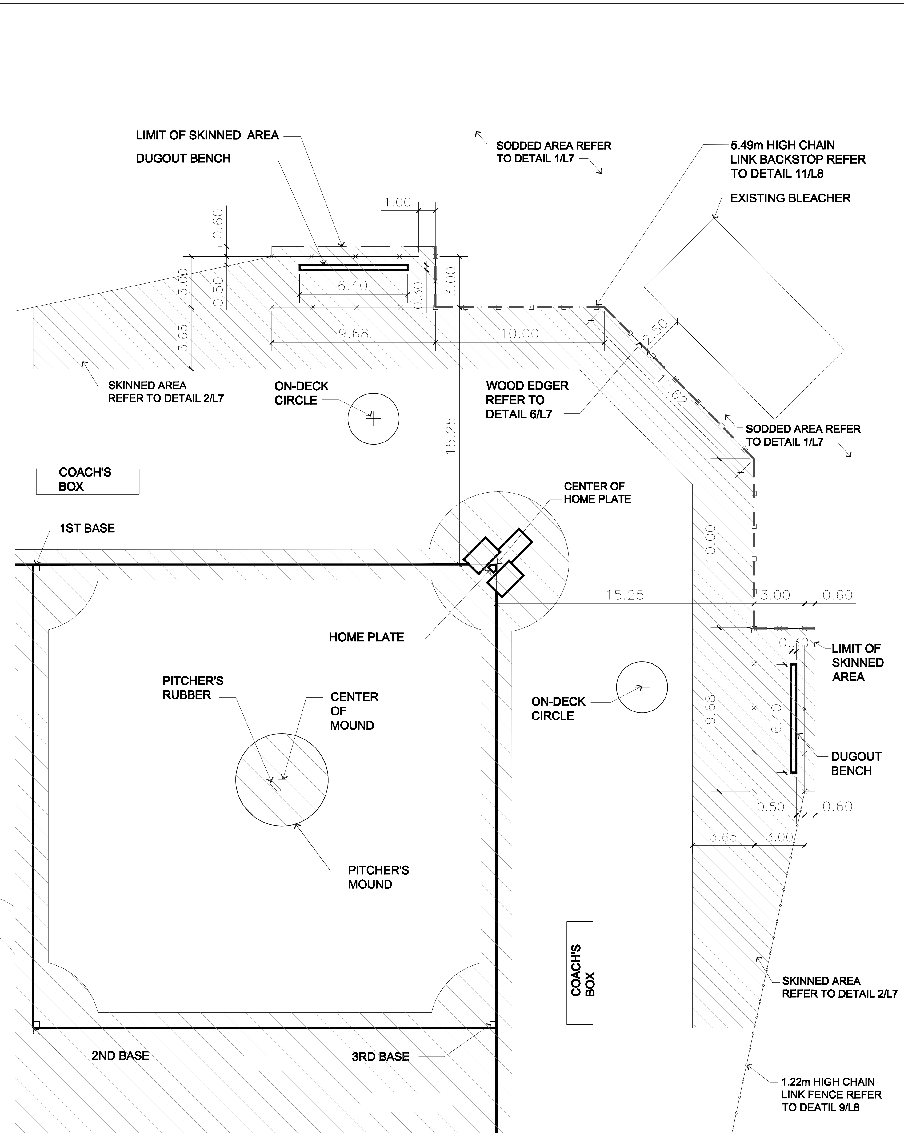
BASEBALL BACKSTOP AREA DETAILS Scale 1:150
