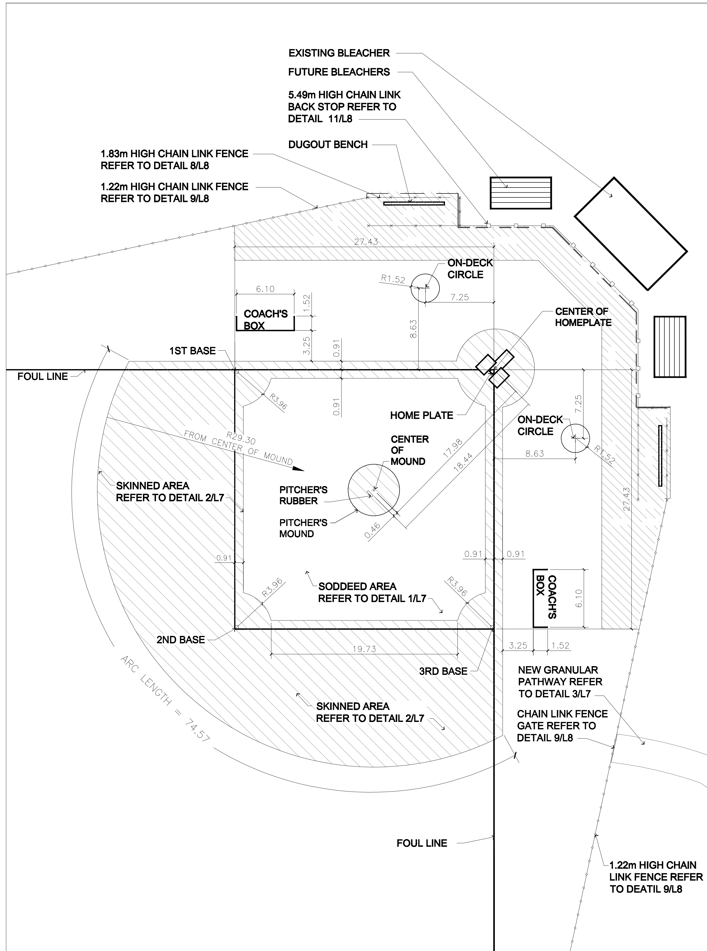
BASEBALL DIAMOND LAYOUT DETAILS Scale 1:200
